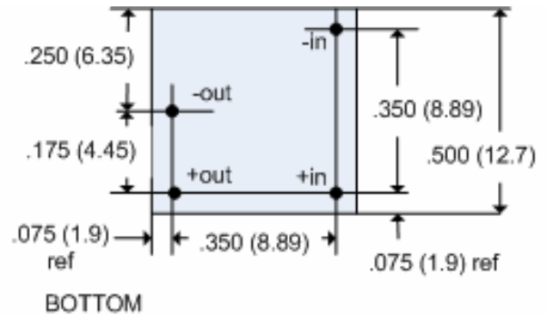
BPS1 - Thru-hole package
